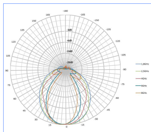
Vertikal Pattern HyperLOG 60xx Series
